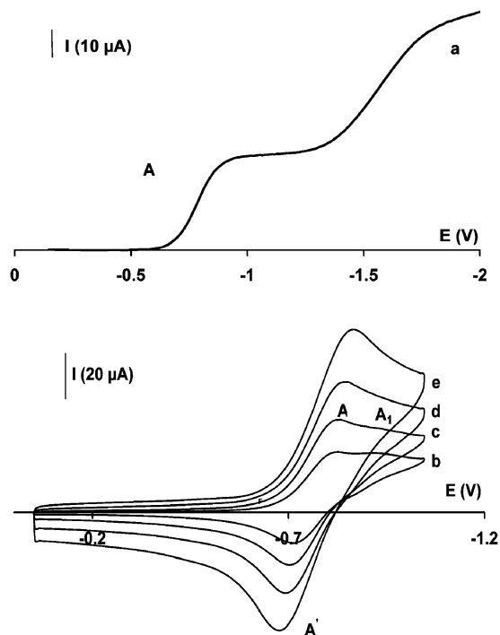
Fig. 2 Voltammograms of complex 2 on carbon electrode in THF containing 0.2 \text{ mol L}^{-1} \text{NBu}_4\text{PF}_6 by RDE voltammetry (a, scan rate: 20 \text{ mV s}^{-1} ) or by CV (b–e) at scan rates: (b): 20 \text{ mV s}^{-1} ; (c): 50 \text{ mV s}^{-1} ; (d) 100 \text{ mV s}^{-1} and (e): 200 \text{ mV s}^{-1} .
