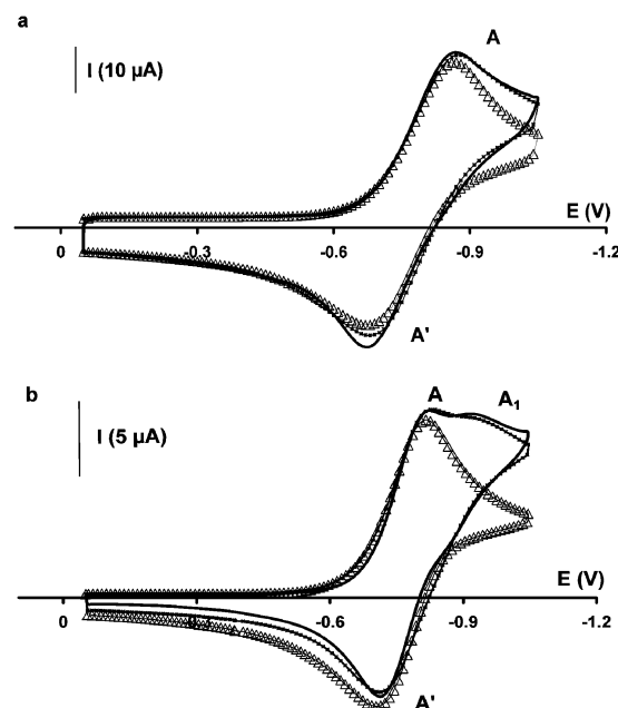
Fig. 4 Cyclic voltammograms of complex 3 on carbon electrode in THF containing 0.2 \text{ mol L}^{-1} \text{NBu}_4\text{PF}_6 : experimental curves (—); simulated curves (■ ■ ■); simulated curves without electronic transfer ( \Delta\Delta\Delta ) at scan rates: (a) 200 \text{ mV s}^{-1} ; (b) 20 \text{ mV s}^{-1} .
