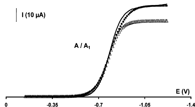
Fig. 3 RDE voltammograms of complex 3 on carbon electrode in THF containing 0.2 \text{ mol L}^{-1} \text{NBu}_4\text{PF}_6 : experimental curves (—); simulated curves (■ ■ ■); simulated curves without electronic transfer ( \Delta\Delta\Delta ) at a scan rate of 20 \text{ mV s}^{-1} and a rotation rate of 104.72 \text{ rad s}^{-1} .
