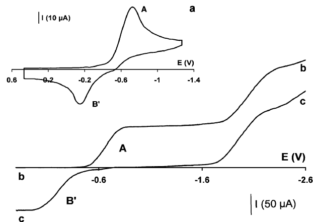
Fig. 1 Voltammograms of complex 1 on carbon electrode in THF containing 0.2 mol \text{L}^{-1} \text{NBu}_4\text{PF}_6 by CV (a, scan rate: 100 \text{mV s}^{-1} ) or by RDE voltammetry (b–c, scan rate: 20 \text{mV s}^{-1} ); (a, b) initial; (c) after electrolysis at -1.20 V ( n = 0.88e^- ).
